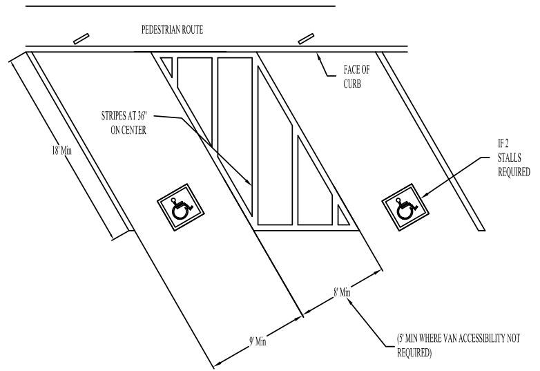
DIAGONAL PARKING
