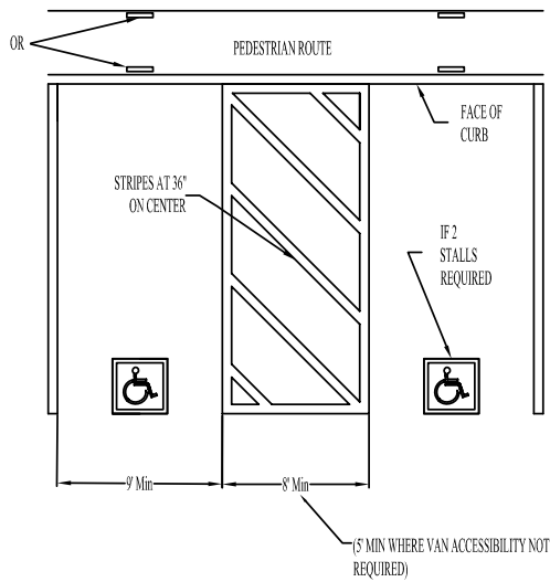
PERPENDICULAR PARKING
