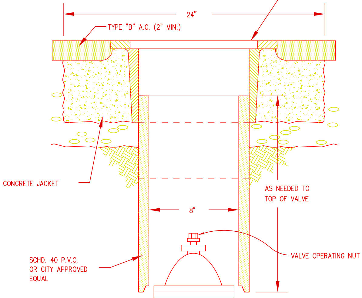
COVER DETAIL
