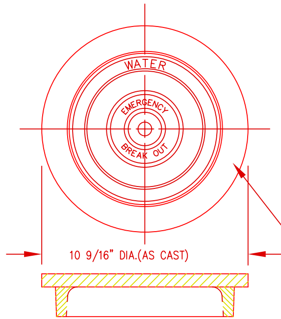
COVER DETAIL
